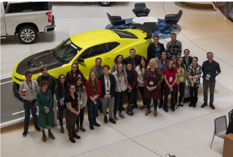
Our Cohort!
